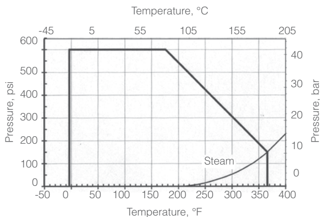
Series DM600 Pressure-Temperature Ratings
