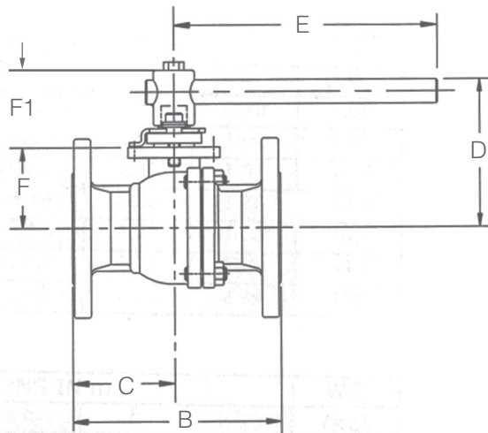
1/2" – 4" Full Port 5801
