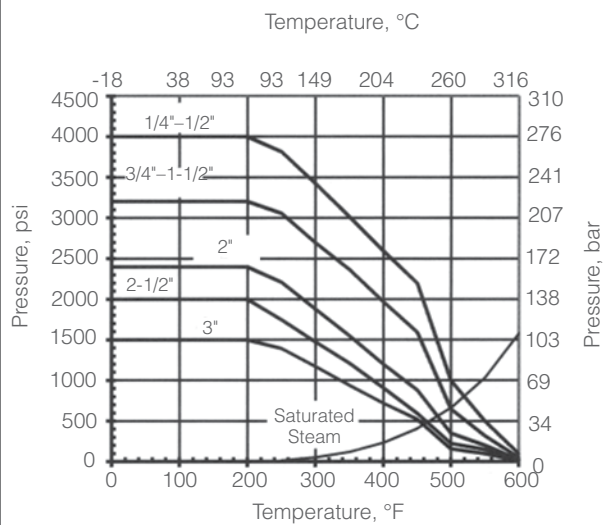
Pressure-Temperature Curves Carbon-Filled PEEK Seats
