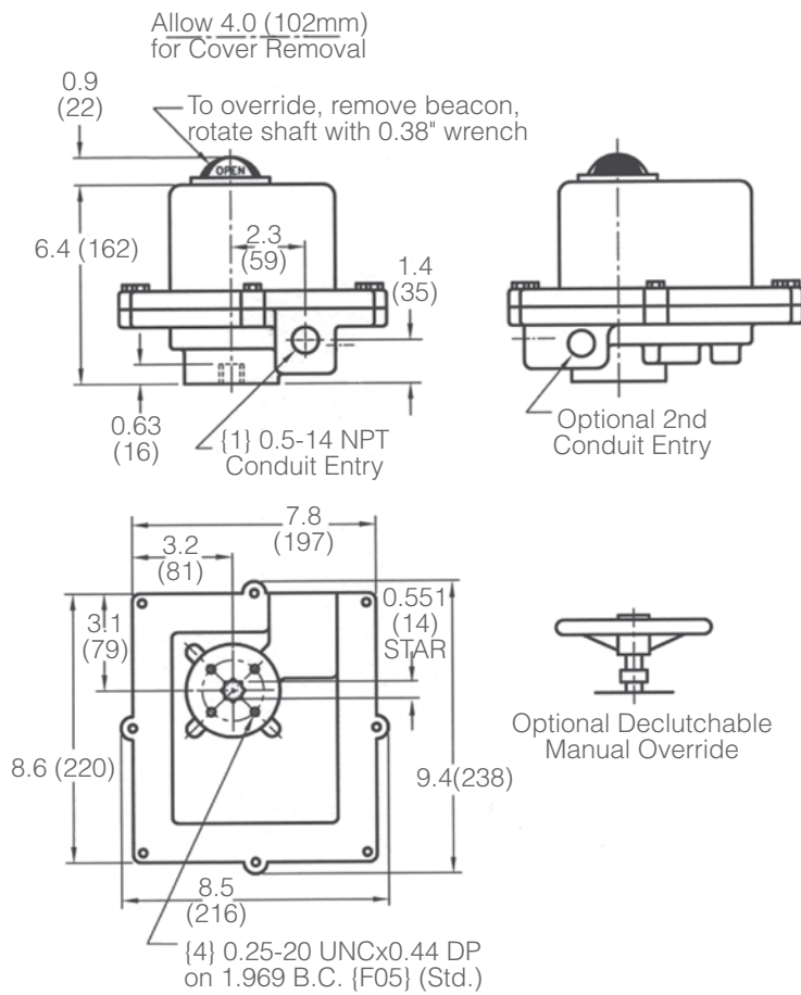
Figure 4 — ER2 & 3 NEMA 4 Large Housing, NEMA 7
