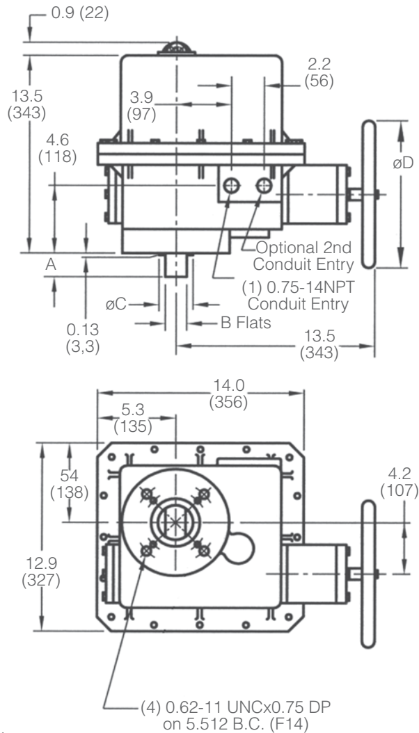
Figure 8 — ER50, 70, 120 & 140
