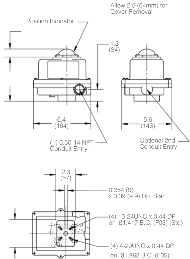
Figure 2 — ER1 NEMA 7
