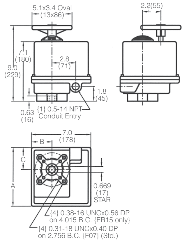
Figure 5 — ER4, 6, 10, 15 NEMA 4
