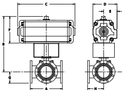
3L/T-2533-150/300 FULL PORT WITH PNEUMATIC ACTUATOR
